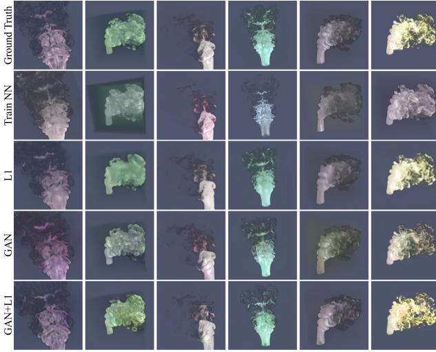
Fig. 13. We compare our method to nearest neighbor retrieval, image-based l_1 loss, and GAN loss for Combustion. Nearest neighbor tends to incorrectly predict color, the l_1 loss blurs details, and the GAN loss can result in color shifts. GAN+L1 strikes a balance between preserving detail and color.
