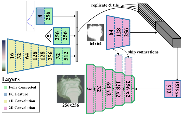
Fig. 5. The generator for the opacity-to-color translation GAN, with symbols and notation consistent with Fig. 4. Skip connections, or the concatenation of the opacity image’s 2D convolutional encodings onto the input of the color image’s decoding, help enforce spatial consistency in the synthesized color image.
