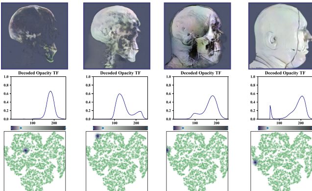
Fig. 11. Exploring the projected latent TF space for Visible Male (bottom) can aid a user's understanding of the space of opacity TFs (middle) based on the synthesized images (top).
