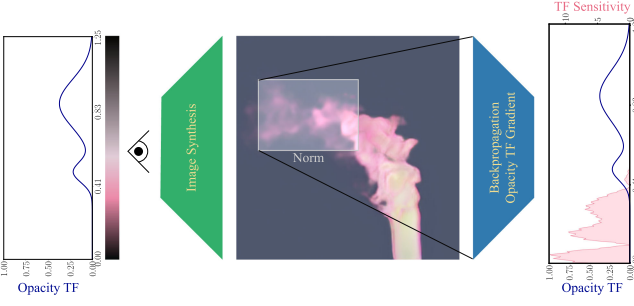
Fig. 6. We illustrate the computation of opacity TF sensitivity. The input parameters are pushed through the network to obtain an image, then the l_2 norm of a user-specified image region is computed, and last the opacity TF gradient is obtained by backpropagation.
