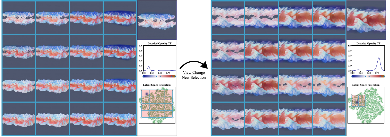
Fig. 10. We show opacity TF exploration through 2D projection of the TF latent space sampling for the Jet dataset. On the left the user selects most of the projection in order to obtain an overview of volumetric features, while still enabling details through direct selection in the projection, shown as the blue Gaussian blob that corresponds to the upper right image and reconstructed TF in the middle right. Selection of a smaller region on the right enables the study of finer-grained shape variation.
