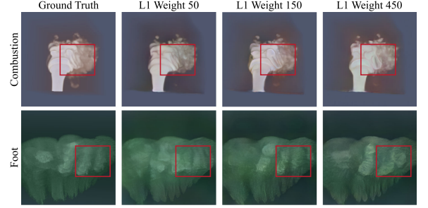
Fig. 15. We compare results in varying the weight of the l_1 loss for Combustion. In certain cases a large weight may fail to preserve detail, while a small weight results in color shift.
